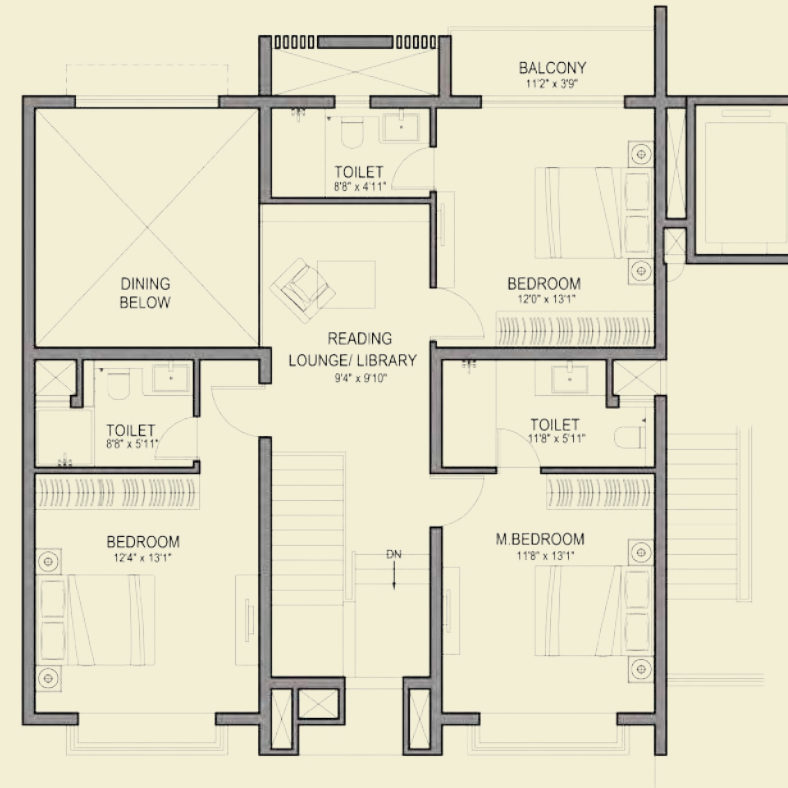
FIRST FLOOR
