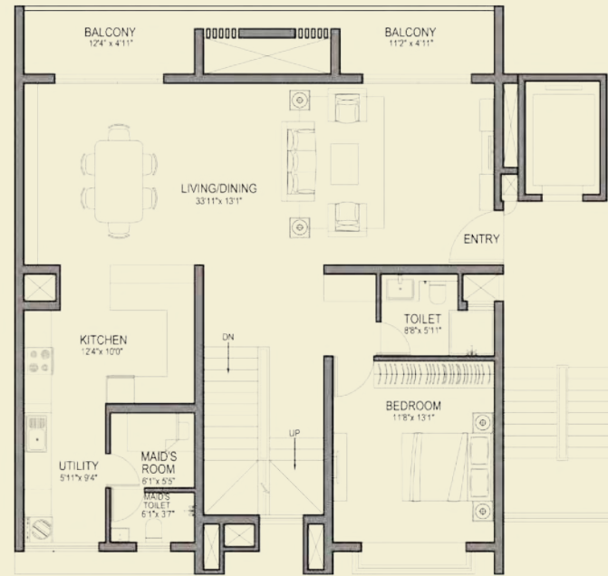
THIRD FLOOR
